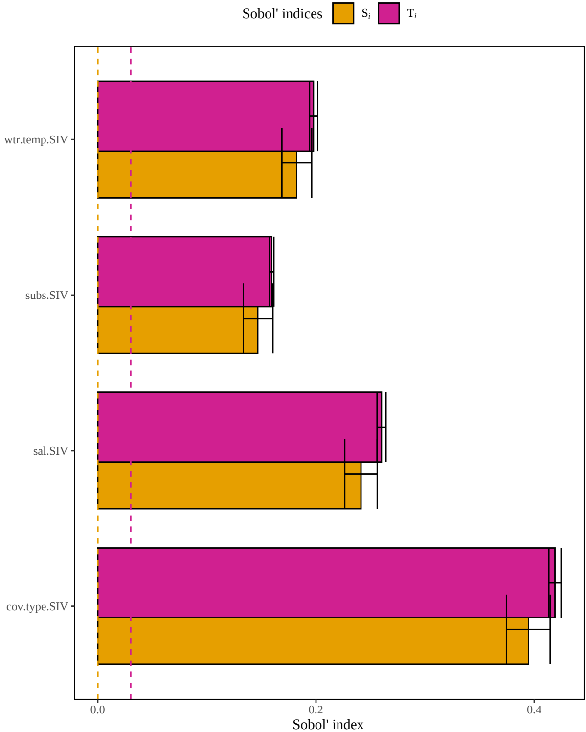
Figure 5. Results of a sensitivity analysis for the pinkshrimpEmergVeg model based on a geometric mean structure. Dashed lines represent baseline numerical approximation error for S_i and T_i ( i.e. , dummy variables).
